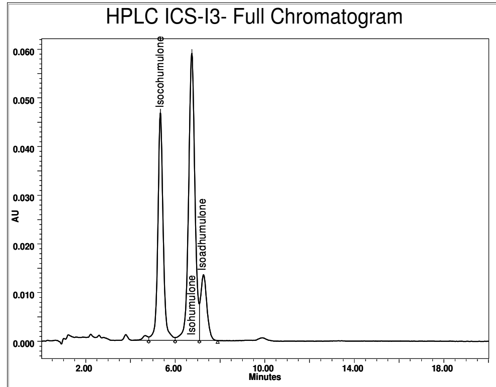
Isohumulone
