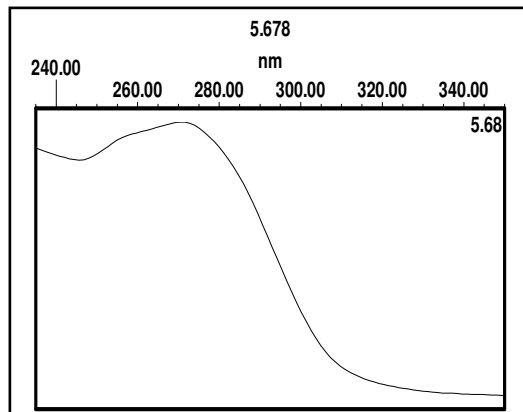
Isocohumulone
