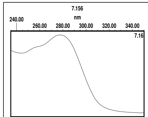
Isohumulone
